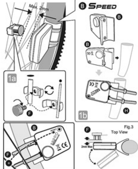
Adjust the distance between transmitter and magnet with max. 2mm as shown in Fig.3.
